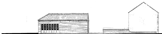
Elevation A - 1:100 as proposed
