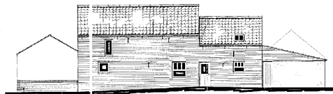
Elevation B - 1:100 as proposed
