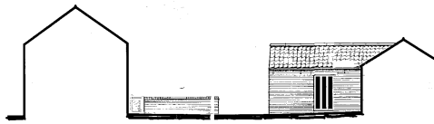
Elevation H - 1:100 as proposed
